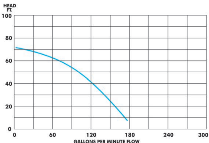
ST3020BCUL Performance Curve 3" Discharge
