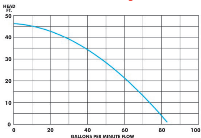
ST2047 Performance Curve 2" Discharge
