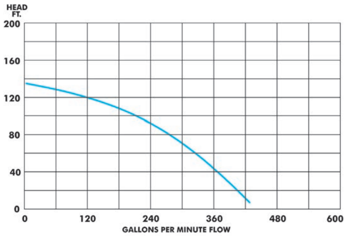
ST41230 Performance Curve 4" Discharge
