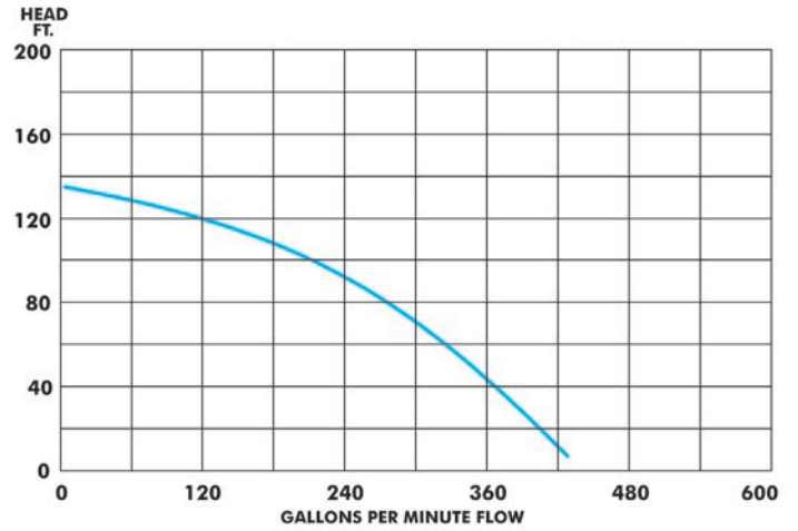
ST41460 Performance Curve 4" Discharge
