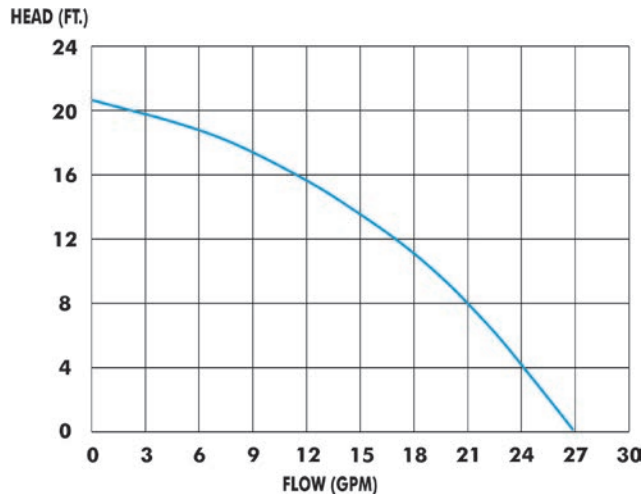
ST1/ST1F Performance Curve 3/4" Discharge
