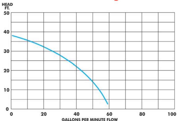
ST2038P Performance Curve 2" Discharge
