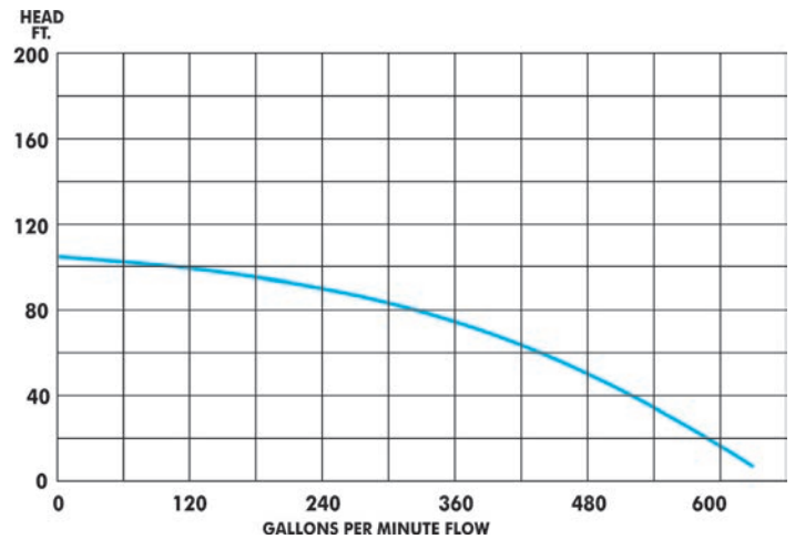
ST61460 Performance Curve 6" Discharge
