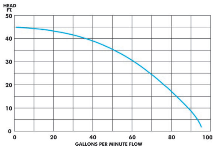
ST2010TCUL Performance Curve 2" Discharge
