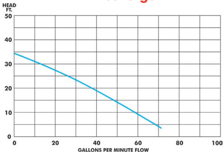
PX400 Performance Curve 2" Discharge
