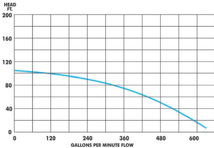
ST61230 Performance Curve 6" Discharge
