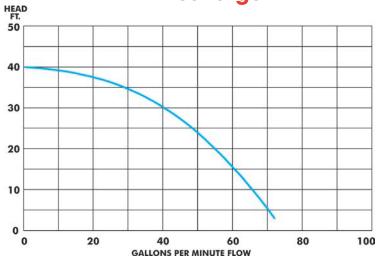
ST2040T Performance Curve 2" Discharge
