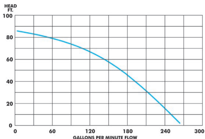
ST3050D Performance Curve 3" Discharge
