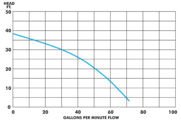
ST2037/ST2037F Performance Curve 2" Discharge
