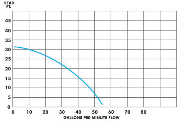
SS233 Performance Curve 2" Discharge
