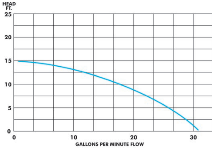
YELLSUB Performance Curve 1 1/4" - 3/4" Discharge
